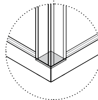
Staffa a terra del montante a scomparsa Ground bracket for concealed posts
